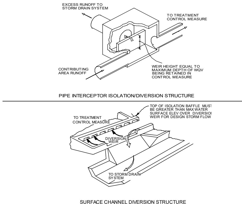
Figure H-1. Common Diversion Structures at Inlets North Tennessee Water Quality BMP Manual Design and Maintenance of Structural BMPs. (2008). (tech.).
