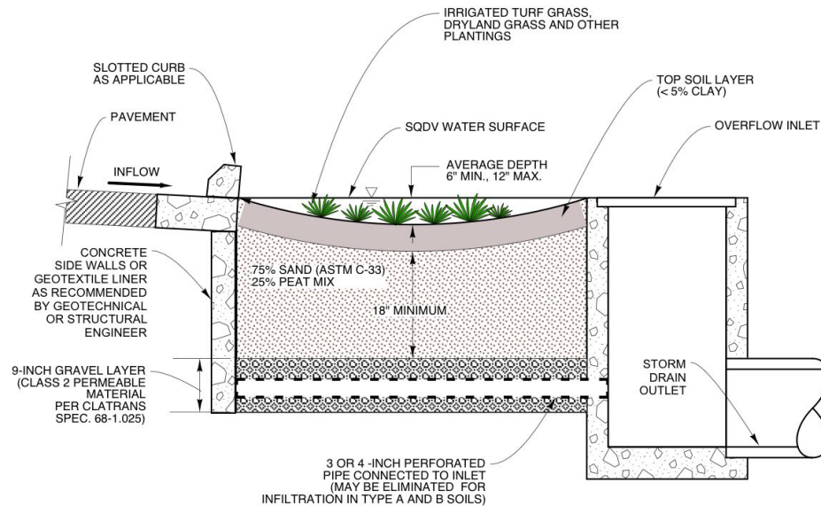
Figure 6-3. Infiltration Stormwater Planter Configuration. Source: Urban Drainage and Flood Control District (UDFCD). (1999, rev. 2008). Drainage Criteria Manual (Vol 3) . Denver, CO.
