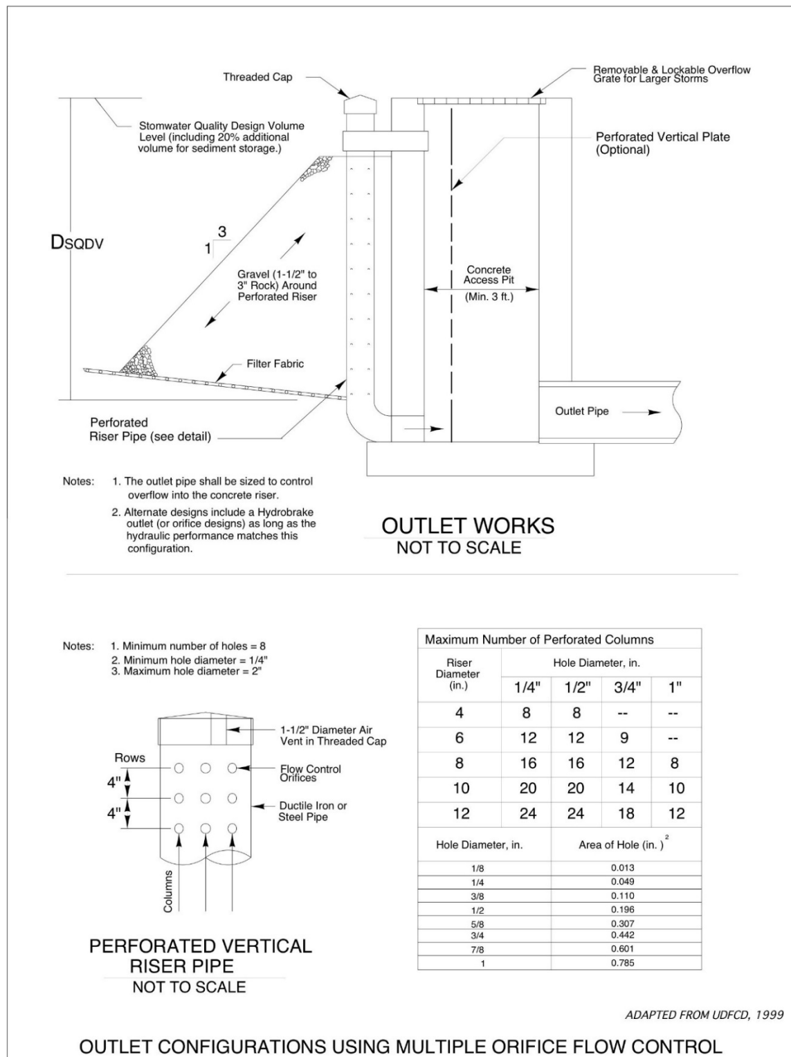
Figure 6-8. Perforated Pipe Outlet Structure. Source: Adapted from Urban Storm Drain Criteria Manual Vol 3. – Best Management Practices, Urban Drainage and Flood Control District. (1999, November).
