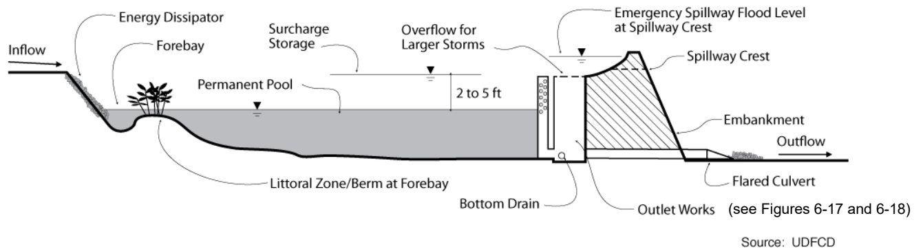
Figure 6-10. Conceptual Layout of Wet Pond. Source: Adapted from Urban Storm Drain Criteria Manual Vol 3. – Best Management Practices , Urban Drainage and Flood Control District. (1999, November).
