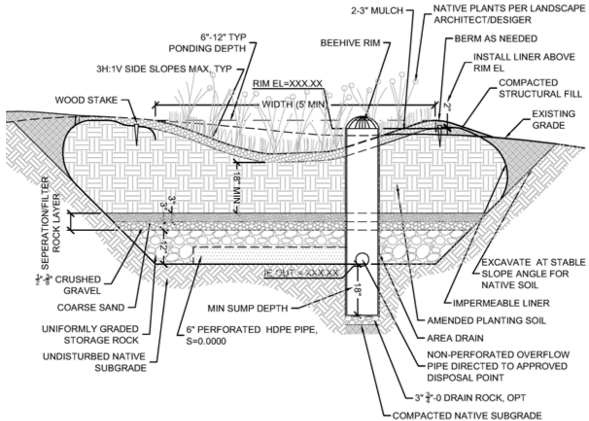
Figure 5-1. Example Rain Garden. Source: Oregon State University. (n.d.). Choose the right Rain Garden. Retrieved October 6, 2021, from https://extension.oregonstate.edu/node/119221/printable/print .
