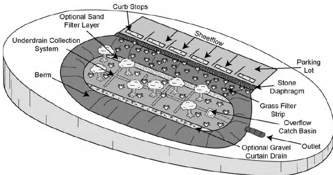
Figure 6-2a. Bioretention Schematic.
