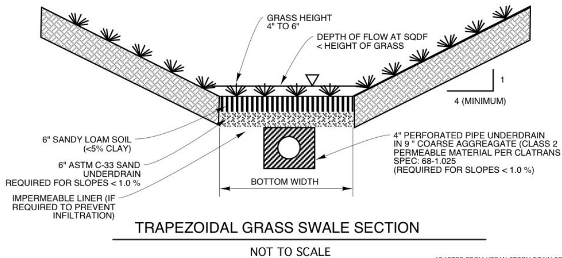
Figure 6-13. Grassy Swale. Source: Adapted from Urban Storm Drain Criteria Manual Vol. 3 – Best Management Practices, Urban Drainage and Flood Control District. (1999, November).
