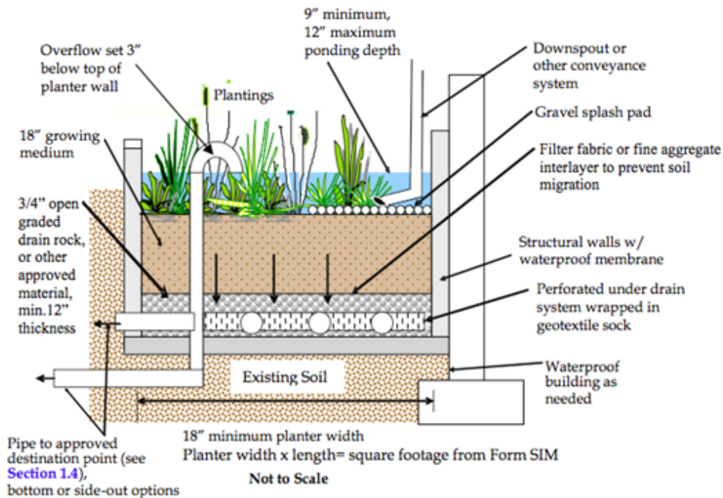
Figure 6-4. Flow-through Stormwater Planter Configuration. "Stormwater Planters." Source: Stormwater Management Manual . [Eugene, Or.]: City of Eugene. (2008). 2-58--62. Print. http://ceppcontent.eugene1.net;7087/publishedcontent/publish/pw/stormwater/docs/ch2e.pdf
