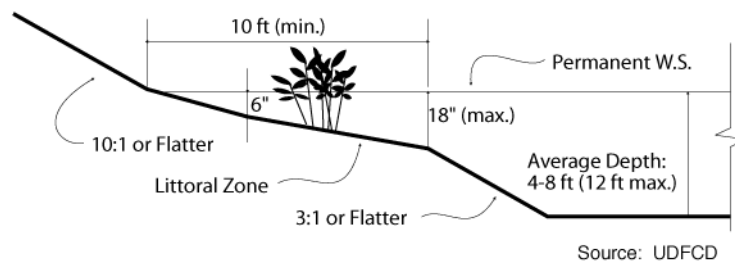
Figure 6-11. Depth Zones for Wet Pond. Source: Adapted from Urban Storm Drain Criteria Manual Vol 3 – Best Management Practices , Urban Drainage and Flood Control District. (1999, November)
