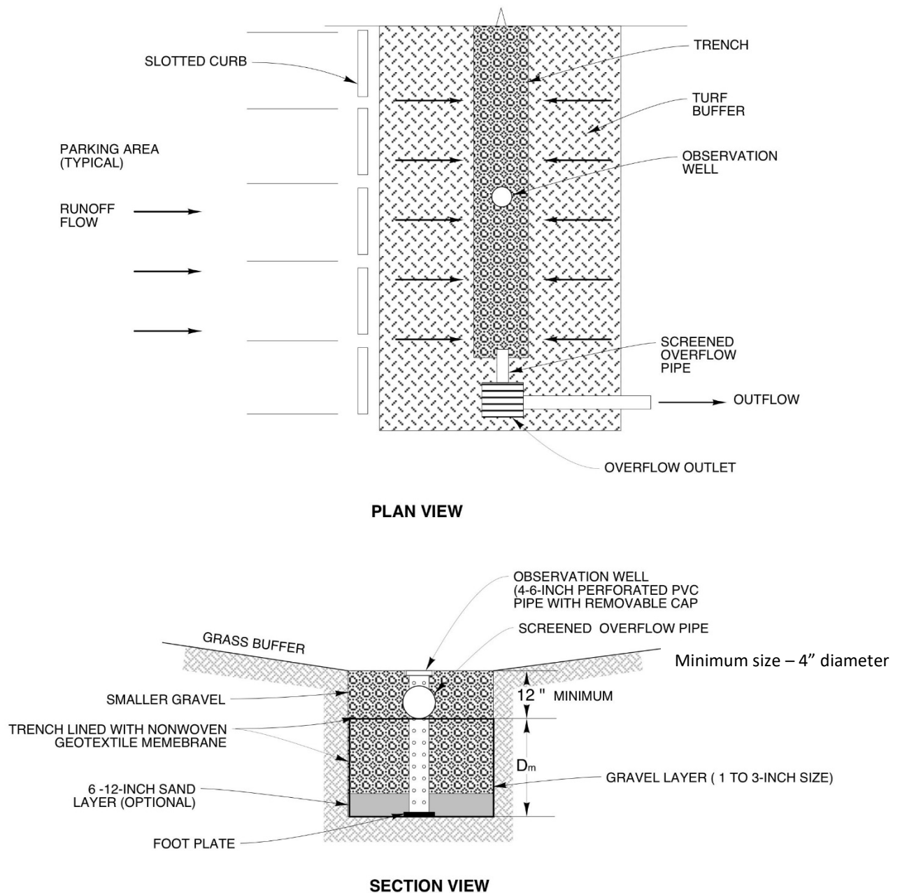
Figure 6-7. Infiltration Trench. Source: Adapted from Urban Storm Drain Criteria Manual Vol 3. – Best Management Practices, Urban Drainage and Flood Control District. (1999, November)
