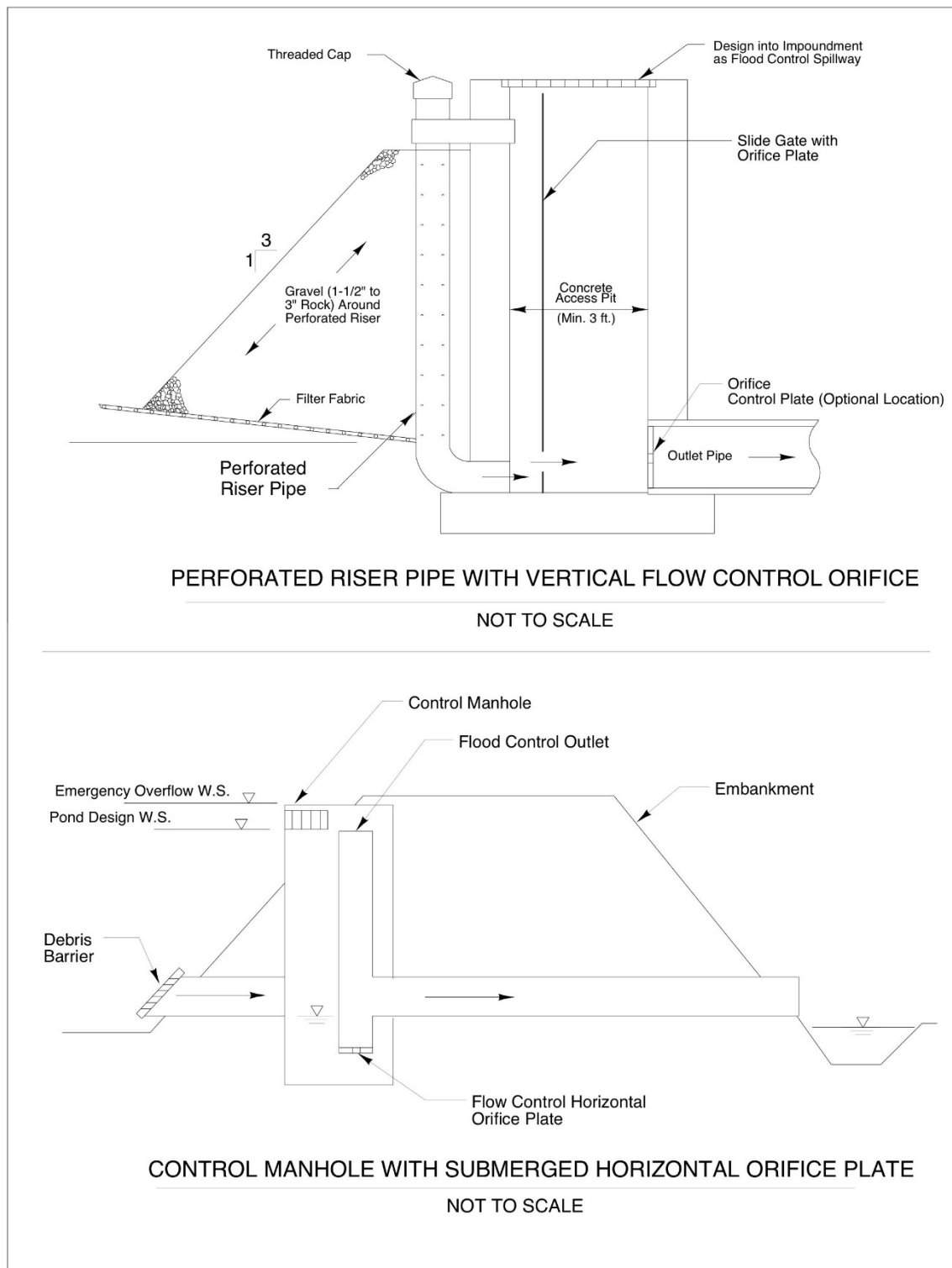
Figure 6-9. Orifice Plate Outlet Configuration. Source: Adapted from Urban Storm Drain Criteria Manual Vol 3. – Best Management Practices, Urban Drainage and Flood Control District. (1999, November).
